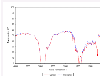
Infrared Spectrum
